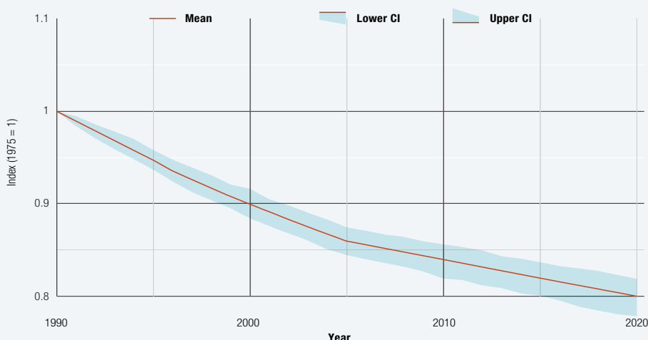
Figure 3 Mediterranean WET Index 1990-2020.
